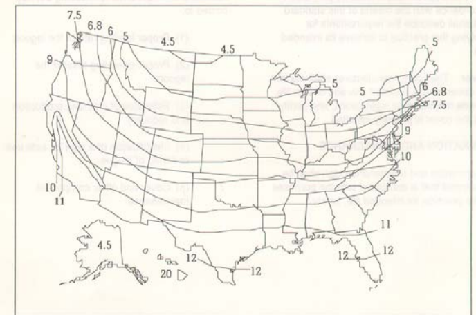
Figure 1: Covered Anaerobic Lagoon Maximum Loading Rate (lb VS/1000ft 2 /day)
