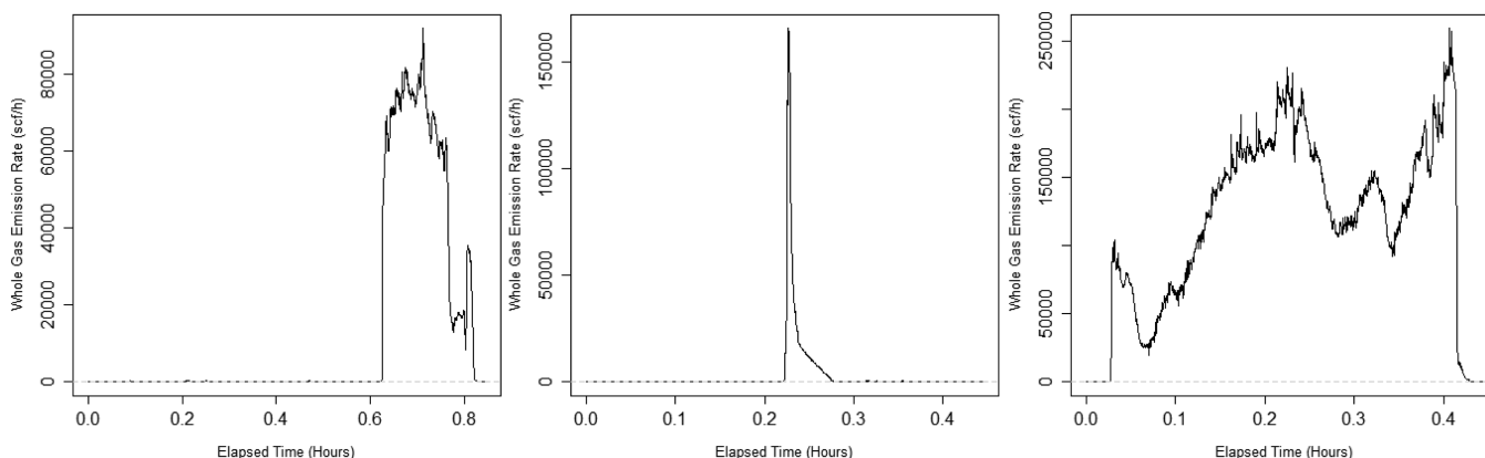
Figure 3. Representative time series of methane flow rates during manually triggered liquid unloadings from wells with plunger lifts (UBB-45-0101 left; UJR-46-0601 middle; USH-45-0202 right); Note differences in horizontal and vertical scales.
